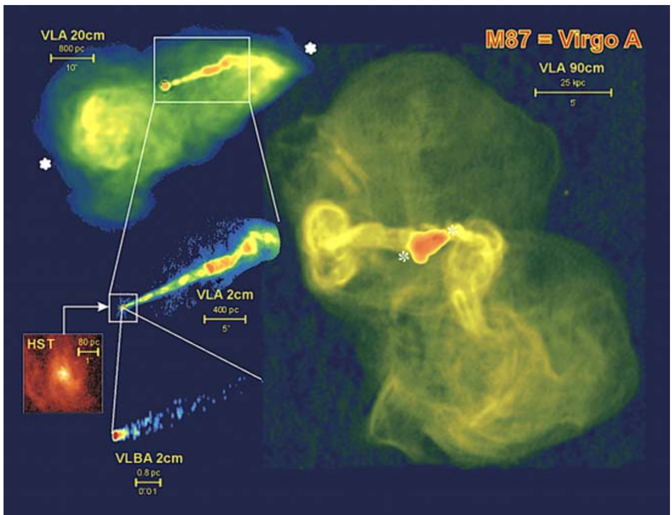
M87 radio- NRAO Very Large Array (VLA), Very Long Baseline Array (VLBA), Hubble Space Telescope (HST) – Radio montage compared to HST image showing large bubbles of energized plasma generated by a pair of opposing jets. Image courtesy of NRAO/AUI.
