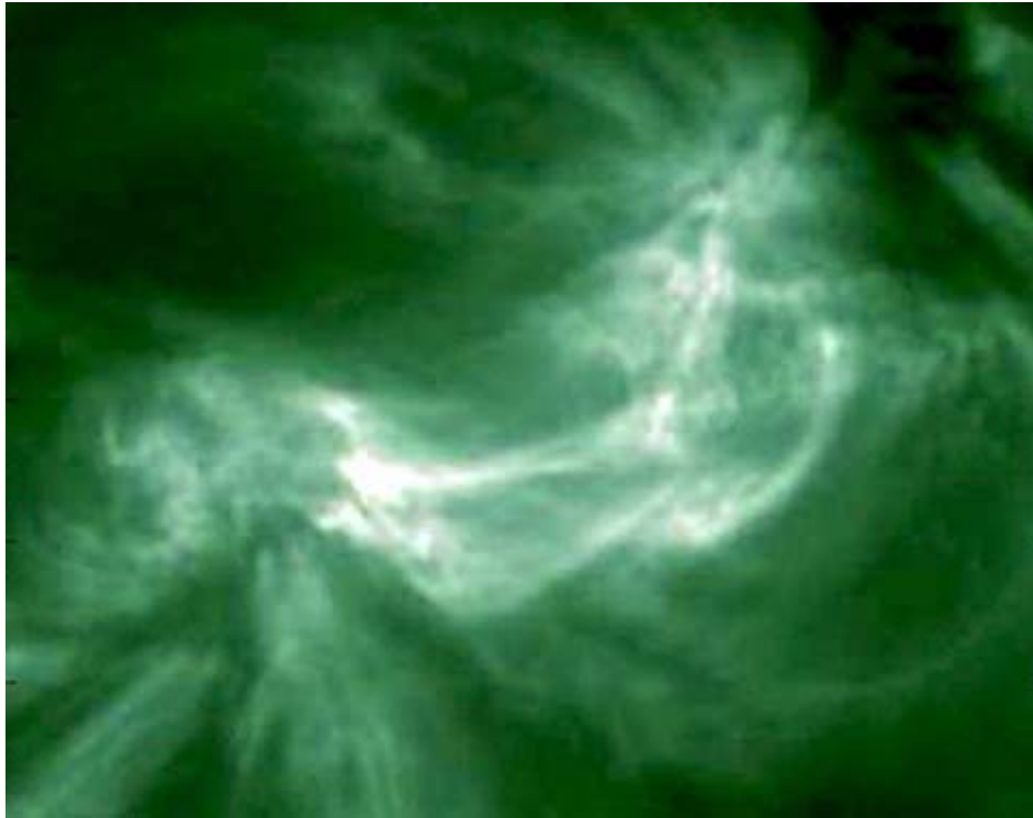
A coronal loop from the Solar Dynamics Observatory. The image covers about fifty thousand miles of the Sun. PHOTO CREDIT: Reale et al. 2019
