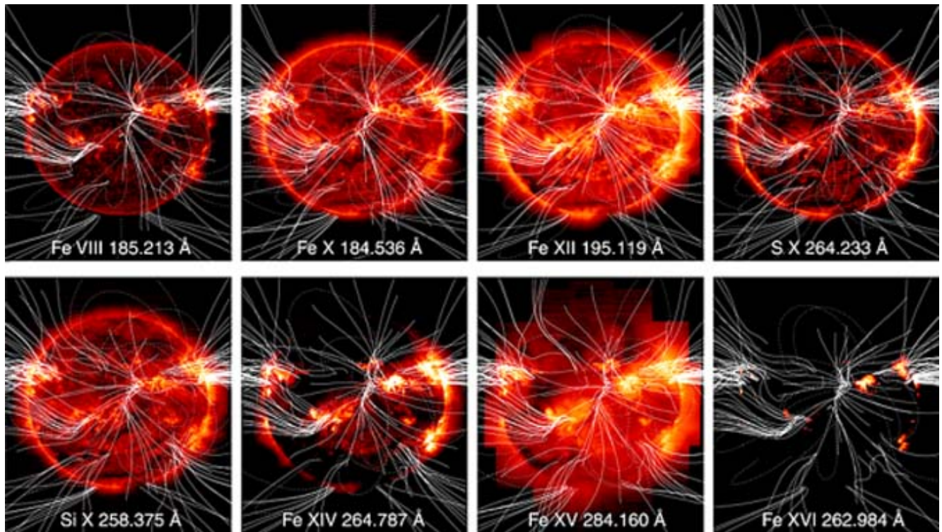
The Sun in various ionization bands. Credit: David H Brooks, Ignacio Ugarte-Urra, Harry P Warren.
